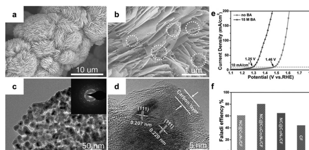
Fig. 3 (a–d) Structural characterization of NC@CuCo 2 N x /CF. (e) LSV curves of OER and BOR. (f) faradaic efficiency of BOR using different catalysts. Reproduced with permission from ref. 86. Copyright 2017 Wiley-VCH.
