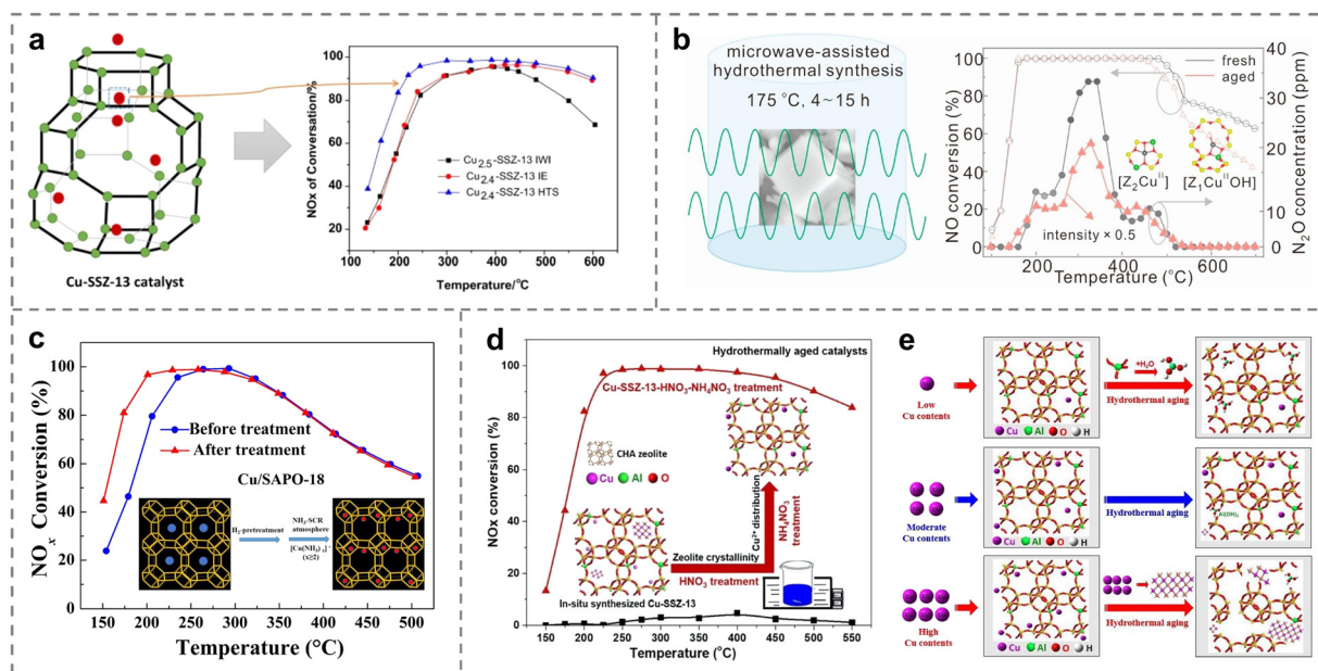
Fig. 8 (a) \text{NH}_3 -SCR performance of various as-prepared catalysts with different preparation methods. Copied with permission from ref. 112. Copyright 2019, Springer Nature. (b) Microwave synthesis conditions and hydrothermal performance of the catalysts. Copied with permission from ref. 113. Copyright 2021, Elsevier. (c) \text{NH}_3 -SCR activity of various Cu/SAPO-18 catalysts with different treatments. Copied with permission from ref. 116. Copyright 2019, Elsevier. (d) \text{NH}_3 -SCR performance of various Cu-SSZ-13 zeolites with different treatments. (e) The deactivation mechanism of Cu-SSZ-13 with different Cu loadings during hydrothermal treatment. Copied with permission from ref. 117. Copyright 2020, Elsevier.
