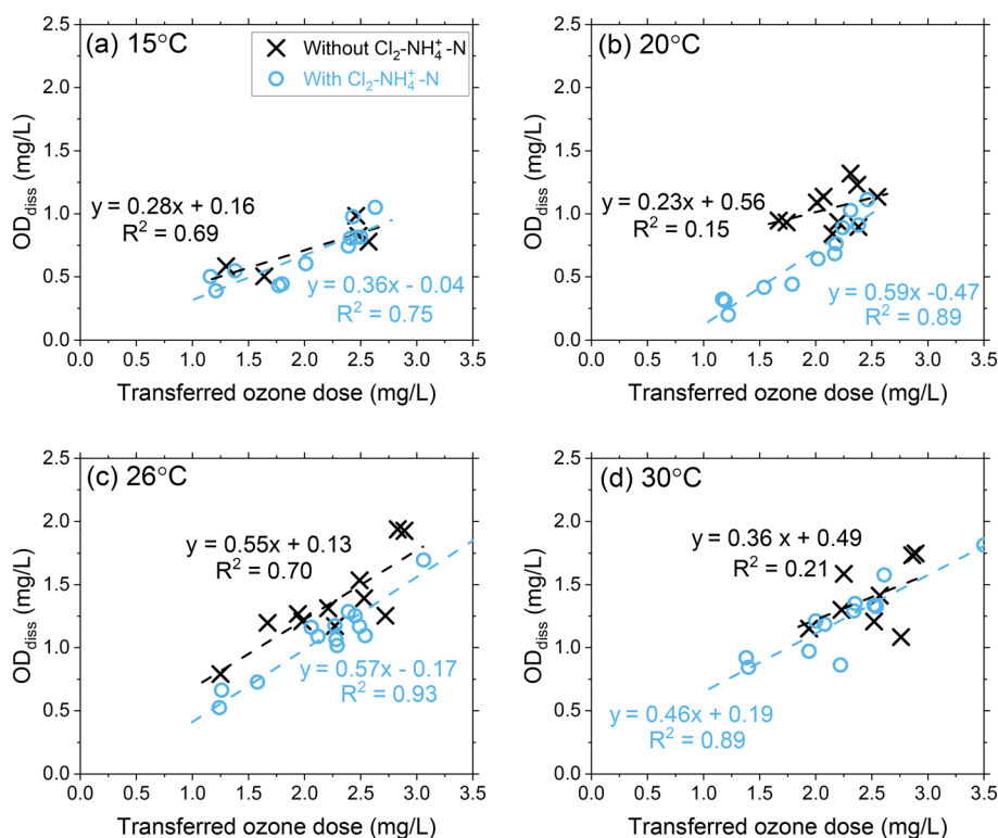
Fig. 2 Pilot-scale data depicting correlations between OD_{diss} as a function of the transferred ozone doses at (a) 15 °C, (b) 20 °C, (c) 26 °C, and (d) 30 °C. Pilot-scale results illustrating the different Cl_2-NH_4^+-N dosing scenarios are presented in Fig. S5.†
