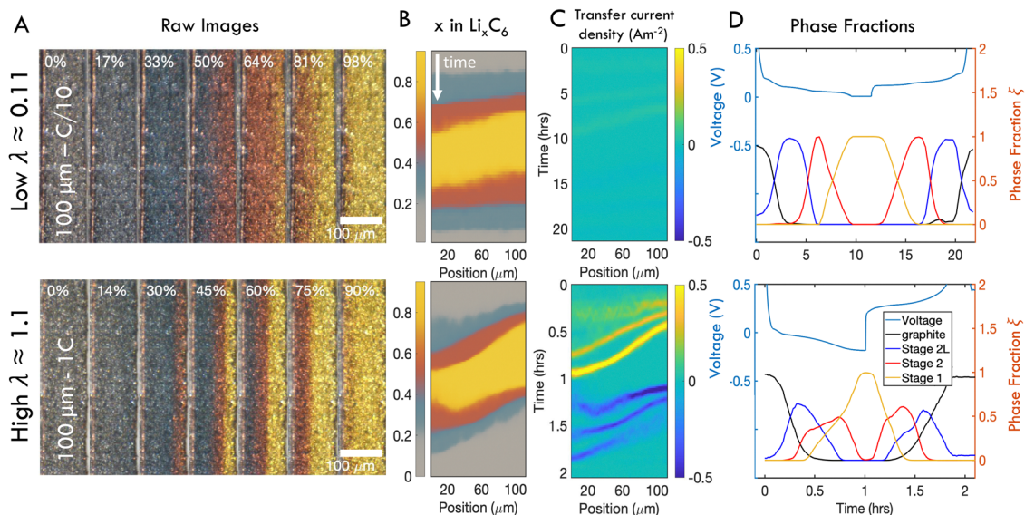
Fig. 4 Representative operando results of "slow" (C/10) and "fast" (1C) charges of 100 μm thick electrodes. (A) Subset of photos taken during charge cycles. In each image, the current collector is located on the left and the separator is on the right. (B) Composite images showing distribution of phases in time and one spatial dimension over a full charge/discharge cycle. (C) Distribution of intercalation current. (D) Anode voltage vs. Li/Li + alongside relative fractions of each phase anywhere in the imaged area as a function of time. At high \lambda , significant overpotentials are accompanied by coexistence of all three phases. Similar figures reporting data from all samples can be found in Fig. S3 and S4 (ESI†).
