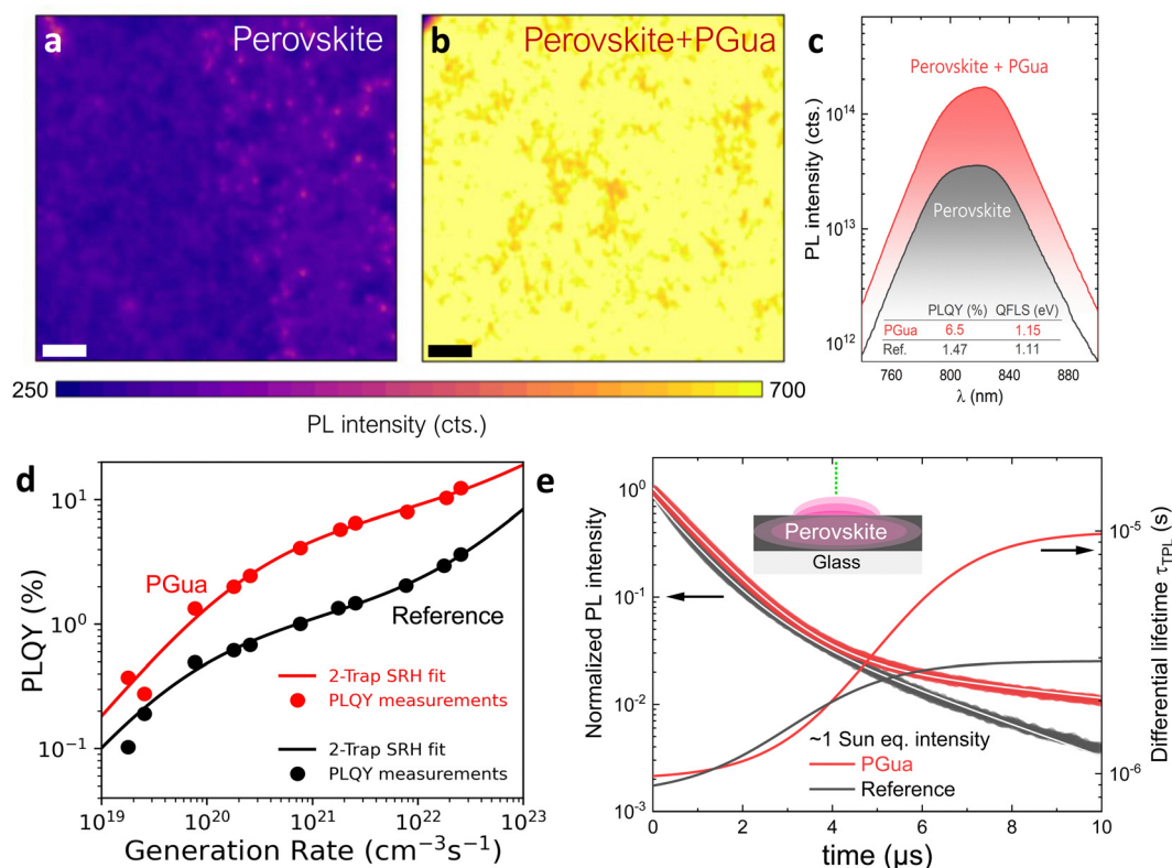
Fig. 2 Opto-electronic properties of perovskite films. Spatially resolved photoluminescence (PL) measurements of (a) reference perovskite film and (b) perovskite films with PGua, scale bar – 6 \mu m. (c) Absolute PL measurement of a reference and PGua-treated perovskite films on glass with respective values for PLQY and QFLS. (d) Generation-dependent PLQY measurements fitted according to a two-trap level SRH model. (e) TRPL measurements of reference and PGua-treated perovskite films at \sim 1 sun equivalent intensity and calculated differential lifetime based on the multi-exponential fits (white lines).
