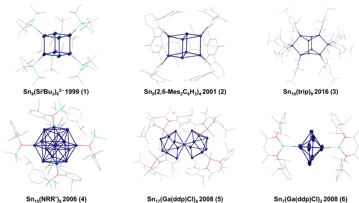
Fig. 1 Overview of metalloid tin clusters synthesized via a reductive approach. Ligands are simplified by wires and sticks (light blue = silicon, light grey = carbon, violet = gallium, green = chlorine, and dark blue = tin).
