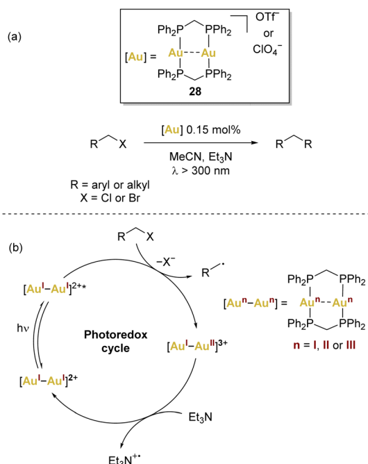
Scheme 6 (a) Che's seminal work using [(\mu\text{-dppm})_2\text{Au}_2]^{2+} ( \text{dppm} = bis(diphenylphosphino)methane), and (b) common proposed mechanism involving complex 28 .
