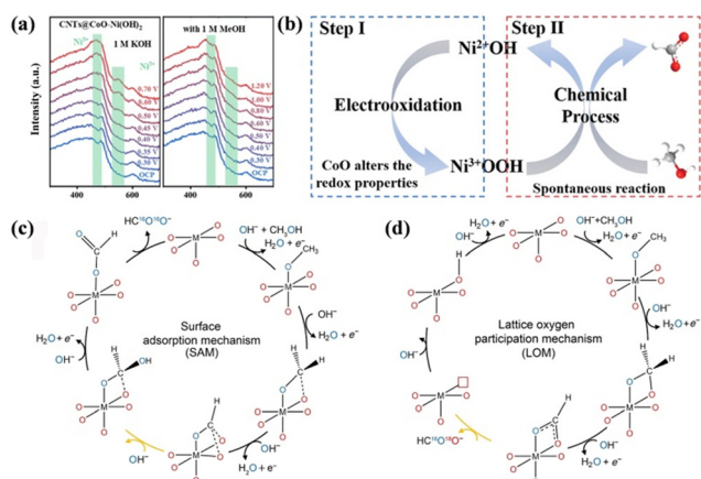
Fig. 2 (a) In situ Raman spectra of the OER and MOR for \text{CNTs@CoO-Ni(OH)}_2 . (b) Dynamic reconstruction of the active \text{Ni}^{3+}\text{OOH} layer. 56 Reproduced from ref. 56 with permission from the Royal Society of Chemistry, Copyright 2023. Possible reaction mechanisms for (c) SAM and (d) LOM. 63 Reproduced from ref. 63 with permission from American Association for the Advancement of Science, Copyright 2023.
