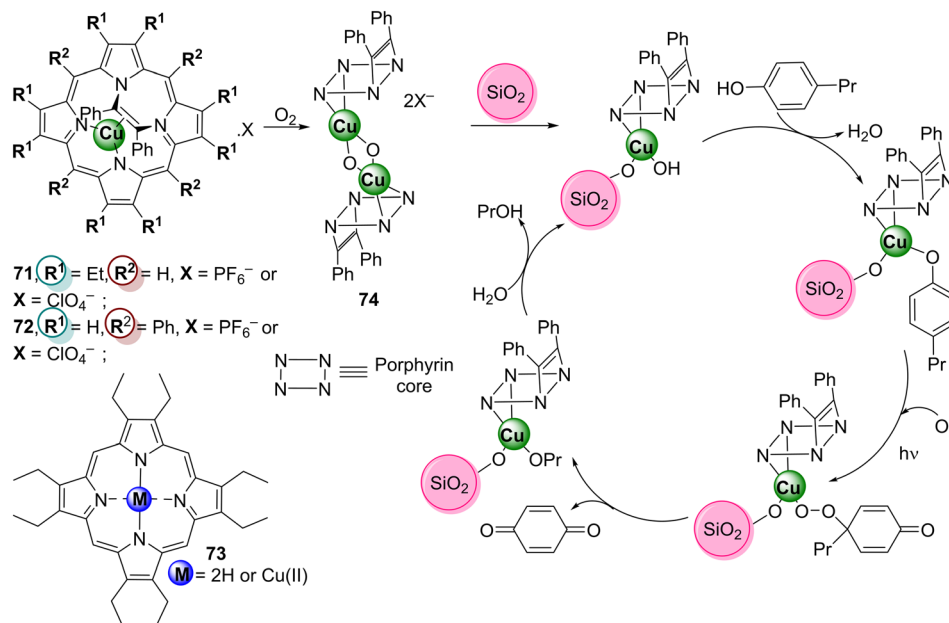
Fig. 25 Copper(I) complexes of the N^{21}, N^{22} -etheno bridged porphyrins 71 and 72 , and the proposed mechanism of the photodegradation of 4-propylphenol catalysed by these complexes immobilized on silica gel.
