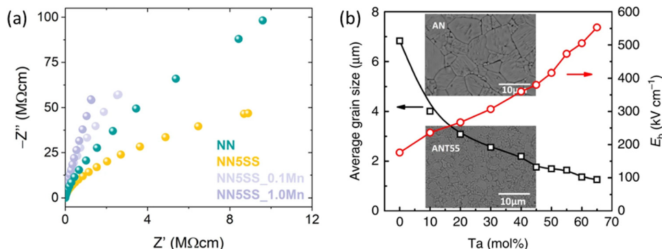
Fig. 21 (a) Nyquist-plot of the NN, NN-5SrSnO 3 , NN-5SrSnO 3 -0.1Mn, and NN-5SrSnO 3 -1.0Mn samples. 49 (b) The composition dependence of average grain size and E_b , the insets give the SEM micrographs of the AN and AN-Ta 0.55 ceramics, respectively. 77 Reprinted with permission ref. 49 from under the terms of the Creative Commons CC BY license, Springer Nature. Reprinted with permission from ref. 77, under the terms of the Creative Commons CC BY license, Springer Nature.
