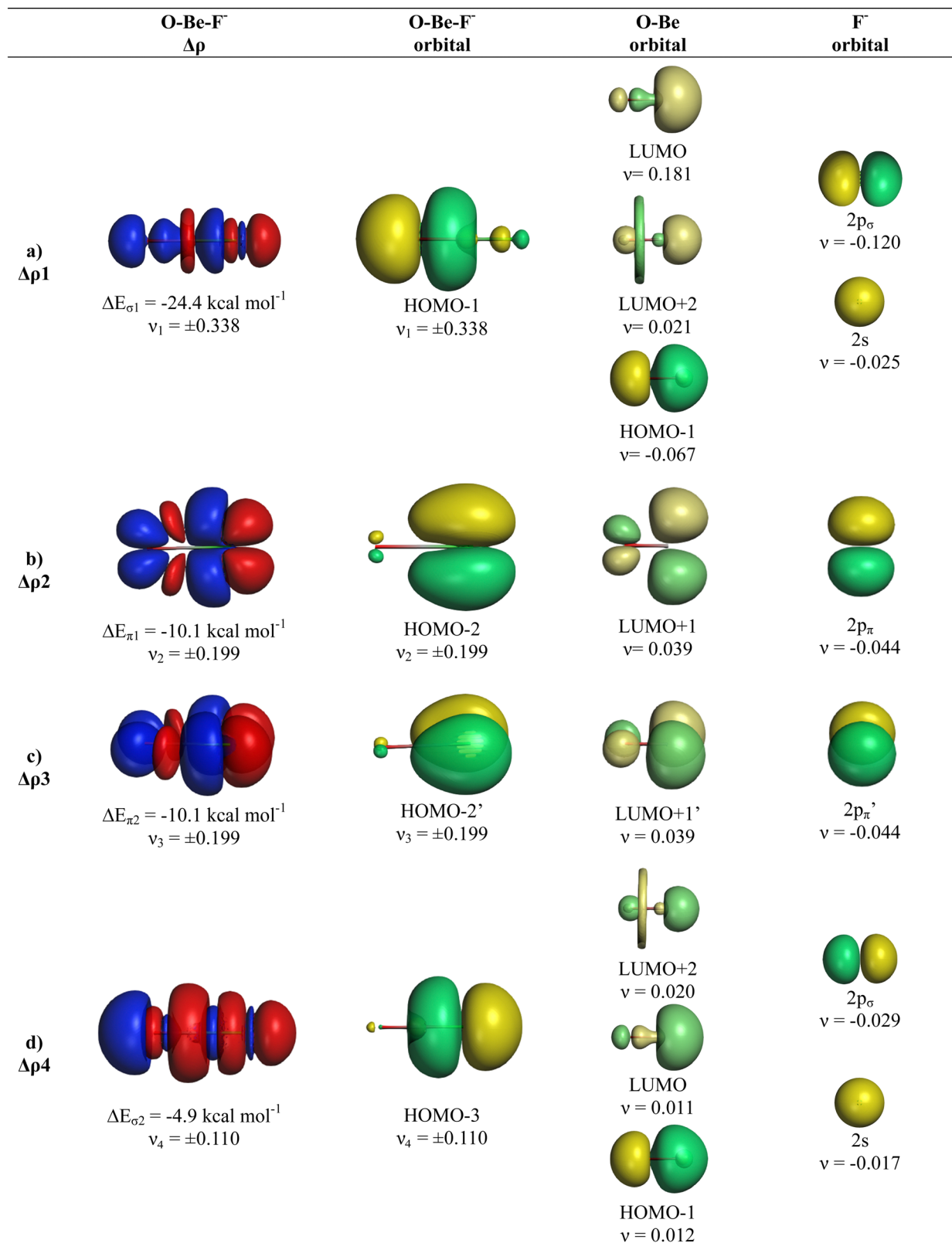
Fig. 4 Plot of deformation densities \Delta\rho of \text{OBeF}^- . The pairwise orbital interactions and the associated interaction energies ( \Delta E_{orb} ) between fragments OBe (S) and \text{F}^- (S) in \text{OBeF}^- at the equilibrium structure as well as the shape of the most important interacting MOs. The direction of the charge flow is red \rightarrow blue. (Isovalue 0.03e \text{ a.u.}^{-3} ).
