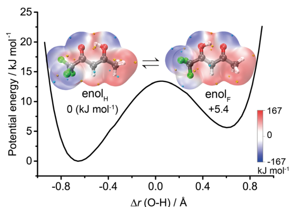
Scheme 1 Schematic illustration of the double minimum potential governing proton transfer along the intramolecular HB between the enol H and enol F forms of trifluoroacetylaceton and the molecular electrostatic potential surfaces.
