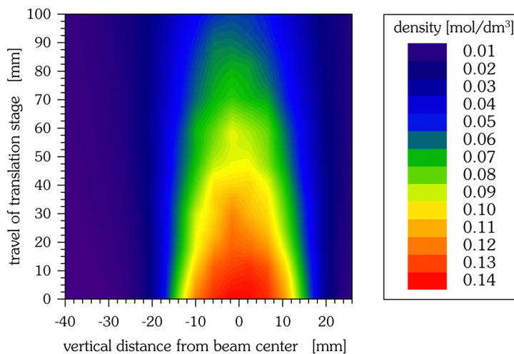
Fig. 7 Particle density of a supersonic helium jet (2.00 MPa, 315.0 K) as obtained from the two-dimensional beam density profile measurements, using the 30 mm detector. Per position, 32 measurements are averaged, each measurement being the average of 50 jet pulses, and with almost 300 positions measured.
