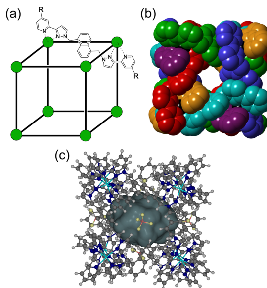
Fig. 1 (a) Cartoon illustrating the cubic host cage [M 8 L 12 ] 16+ , abbreviated as H (R = H), emphasising the cubic array of Co(II) ions and the disposition of one bridging ligand; and its derivatives bearing substituents at the twenty-four externally-directed pyridyl C 4 positions H W (R = CH 2 OH), and H Peg [R = −(CH 2 OCH 2 ) 3 CH 2 OMe]. (b) A view of the complete structure with all ligands shown, coloured differently to emphasise their overall disposition and the presence of portals in the faces. (c) A view of the complete cage structure, highlighting the guest binding cavity space (V = 409 Å 3 ).
