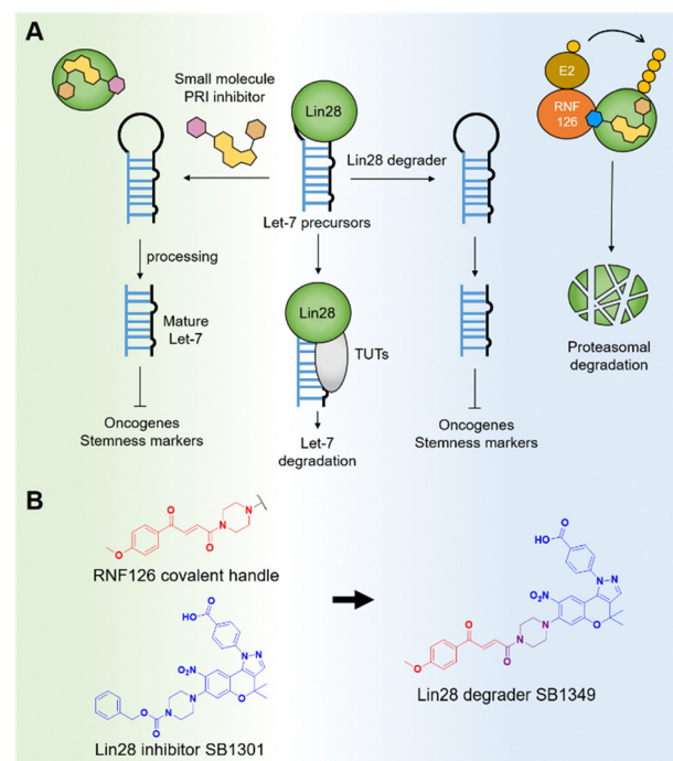
Fig. 1 (A) Schematic diagram of let-7 miRNA biogenesis with a mechanism of Lin28 inhibitor and degrader. (B) Proposed design of a molecular glue-based Lin28 degrader using Lin28–let-7 inhibitor SB1301 with fumarate as a handle for RNF126 E3 ligase.
