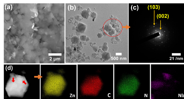
Fig. 1 (a)–(c) Observation of ZIF-8/ \text{Nb}_4\text{C}_3\text{T}_x (75) using SEM (a), TEM (b), and the corresponding SAED pattern (c). The indicated peaks correspond to the diffraction signal of \text{Nb}_4\text{C}_3\text{T}_x . (d) HAADF-STEM image and elemental mapping of ZIF-8/ \text{Nb}_4\text{C}_3\text{T}_x (75).
