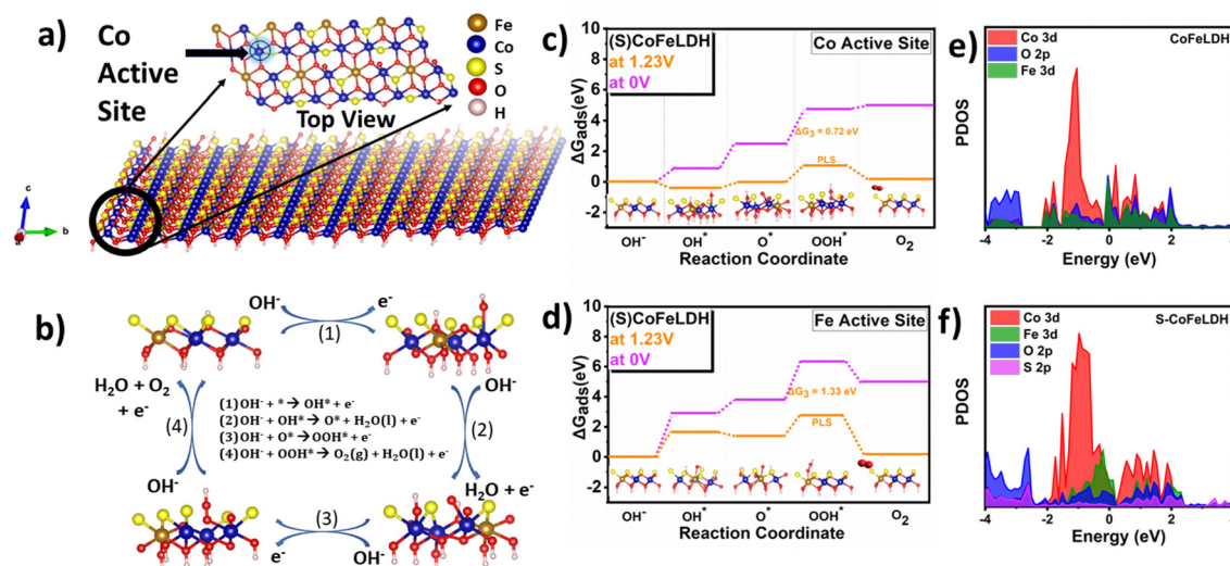
Fig. 6 (a) Theoretically simulated active site illustration. (b) OER mechanism. (c) and (d) Gibbs free energy plot of S-CoFeLDH on Co and Fe active sites, respectively. (e) and (f) PDOS plot of CoFeLDH and S-CoFeLDH.
