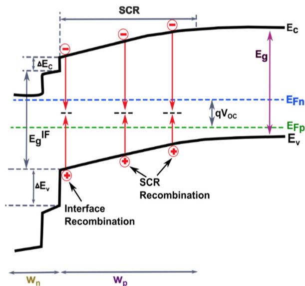
Fig. 8 Schematic presentation of the possible recombination paths of heterostructure \text{Sb}_2\text{Se}_3 solar cells under open-circuit conditions (where E_c , E_v , E_g , E_{\text{Fn}} , E_{\text{Fp}} , E_{\text{giF}} , w_n , w_p , and E_{\text{Fn}}/E_{\text{Fp}} are denoted by the conduction band, valence band, bandgap, interface bandgap, width of the SCR in the buffer layer, width of the SCR in the absorber layer, and quasi-Fermi levels respectively).
