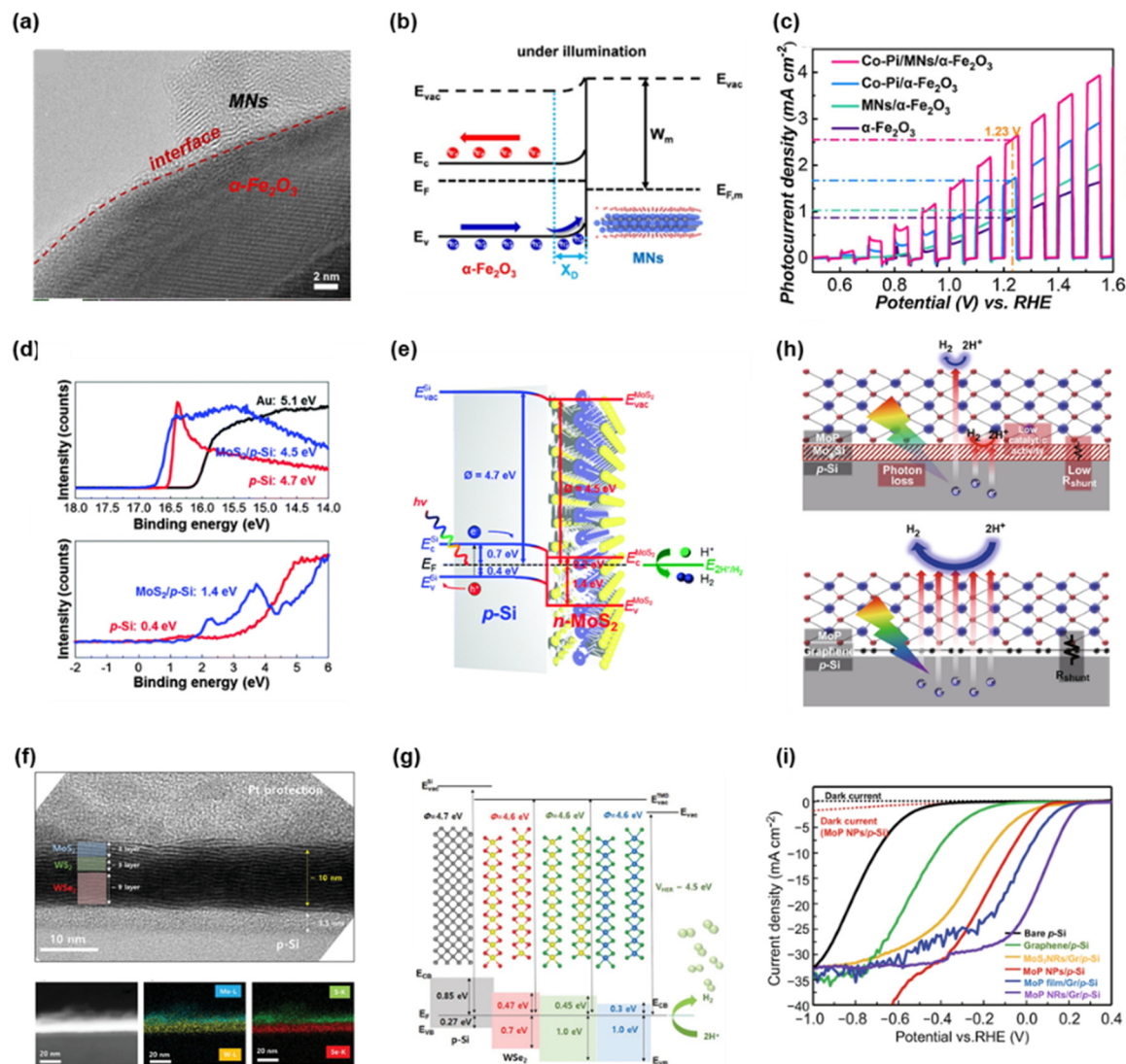
Fig. 3 (a) High-resolution TEM image of MXene nanosheets/ \alpha -Fe _2 O _3 . (b) Energy band diagram of MXene nanosheets/ \alpha -Fe _2 O _3 Schottky junction under illumination. (c) LSV curves of \alpha -Fe _2 O _3 , MNs/ \alpha -Fe _2 O _3 , Co-Pi/ \alpha -Fe _2 O _3 , and Co-Pi/MNs/ \alpha -Fe _2 O _3 . Copyright 2021, Elsevier. (d) UPS and XPS spectra of Au, p-Si, and MoS _2 /p-Si. (e) Schematic of energy band diagram of the MoS _2 /p-Si photocathode having p-n junction. Copyright 2016, Royal Society of Chemistry. (f) Cross-sectional high-resolution TEM image for 112-MWW/p-Si thin film. Copyright 2019, Wiley-VCH GmbH. (g) Schematic of energy band diagram of 112-MWW/p-Si thin film. Copyright 2019, Wiley-VCH GmbH. (h) Schematic of MoP/MoS _2 /p-Si and MoP/graphene/p-Si. (i) LSV curves of bare p-Si, graphene/p-Si, MoS _2 NRs/Gr/p-Si, MoP NPs/p-Si, MoP film/Gr/p-Si, and MoP NRs/Gr/p-Si. Copyright 2021, Springer Nature.
