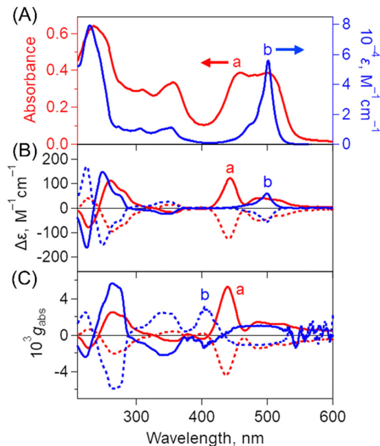
Fig. 4 (A) Absorption spectra of (a) (0Ph-B-BODIPY) m in H 2 O/THF = 99/1 ( v/v ). [0Ph-B-BODIPY] = 30 \mu\text{M} and (b) 0Ph-B-BODIPY in THF. [0Ph-B-BODIPY] = 30 \mu\text{M} . (B) CD spectra of (a) (0Ph-B-BODIPY) m in H 2 O/THF = 99/1 ( v/v ). [0Ph-B-BODIPY] = 30 \mu\text{M} and (b) 0Ph-B-BODIPY in THF. [0Ph-B-BODIPY] = 30 \mu\text{M} . Solid and dotted lines correspond to S and R forms, respectively. (C) Dissymmetry factor g_{\text{abs}} profiles of (a) (0Ph-B-BODIPY) m in H 2 O/THF = 99/1 ( v/v ). [0Ph-B-BODIPY] = 30 \mu\text{M} in H 2 O/THF and (b) 0Ph-B-BODIPY in THF. Solid and dotted lines correspond to S and R forms, respectively.
