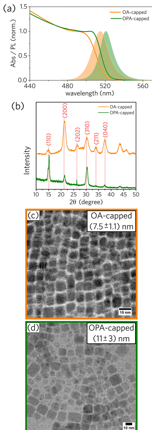
Fig. 1 (a) Absorption and PL emission spectra for OA-capped and OPA-capped \text{CsPbBr}_3 PNCs (OA: oleic acid, OPA: oleylphosphoric acid). (b) Diffraction patterns for OA-capped and OPA-capped \text{CsPbBr}_3 PNCs with diffraction patterns corresponding to an orthorhombic. TEM images for (c) OA- and (d) OPA-capped \text{CsPbBr}_3 PNCs.
