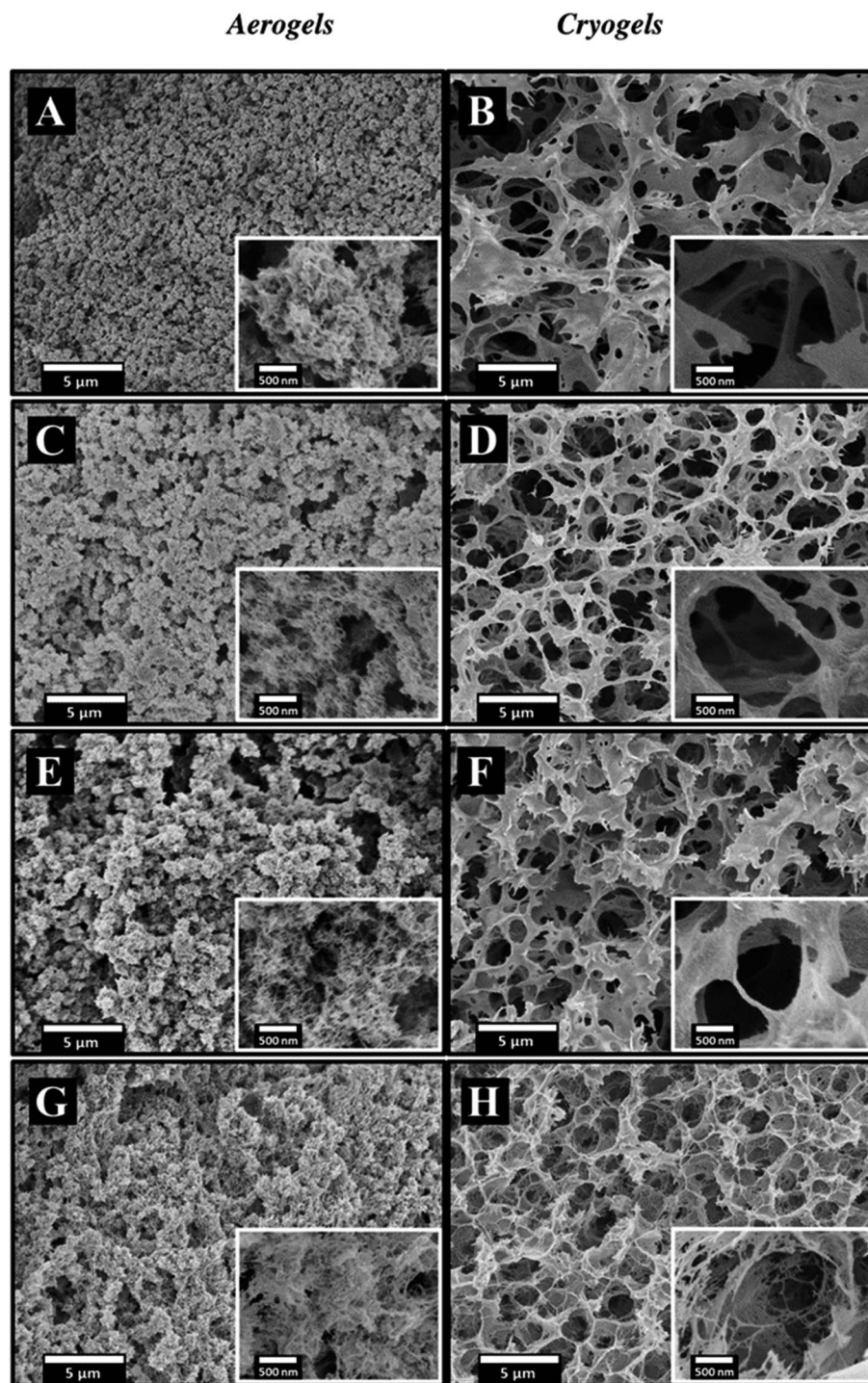
Fig. 6 Morphology of aerogels (A, C, E and G) and cryogels (B, D, F and H) from MCC (A and B), rayon (C and D), viscose (E and F) and cotton (outside macrovoids) (G and H) dissolved in [DBNH][OAc]/DMSO and coagulated using method 1.
