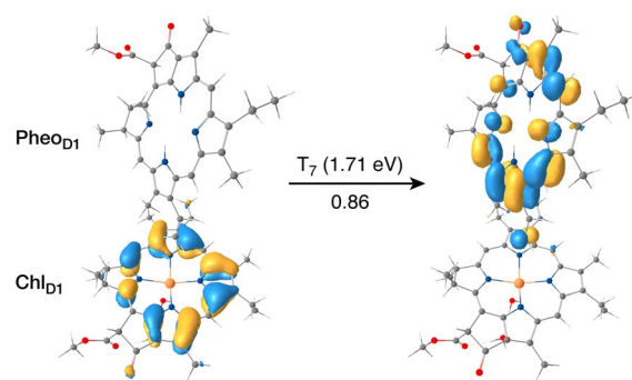
Fig. 4 The identity of the triplet excited state with significant [ \text{Chl}_{\text{D1}}^{\delta^+}\text{Pheo}_{\text{D1}}^{\delta^-} ] charge transfer character in terms of canonical molecular orbitals and their contribution to the given excitation (calculation performed on the [ \text{P}_{\text{D1}}\text{P}_{\text{D2}}\text{Chl}_{\text{D1}}\text{Pheo}_{\text{D1}} ] tetramer, but only the implicated pigment pair is depicted).
