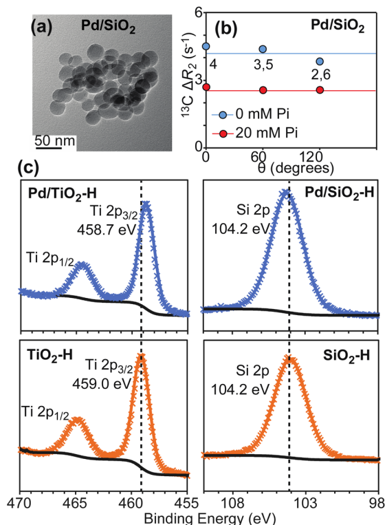
Fig. 7 Properties of Pd/SiO 2 . Panel (a) shows a TEM image for the investigated Pd/SiO 2 material. Panel (b) shows a plot of the 13 C Δ R 2 as a function of θ measured for PhOH in the presence of 1 wt% Pd/SiO 2 . The ortho (2.6) and meta (3.5) positions generate equivalent NMR peaks and one single Δ R 2 value for these peaks is reported. Data measured in the presence of 0 and 20 mM Pi are shown as blue and red spheres, respectively. Solid blue and red lines are the corresponding average Δ R 2 values. Panel (c) shows XPS spectra measured for TiO 2 (bottom left), Pd/TiO 2 (top left), SiO 2 (bottom right), and Pd/SiO 2 (top right) after hydrogen treatment (see ESI Methods † ). The shift of the XPS Ti 2p peaks after hydrogen treatment is consistent with Ti reduction in the presence of supported Pd.
