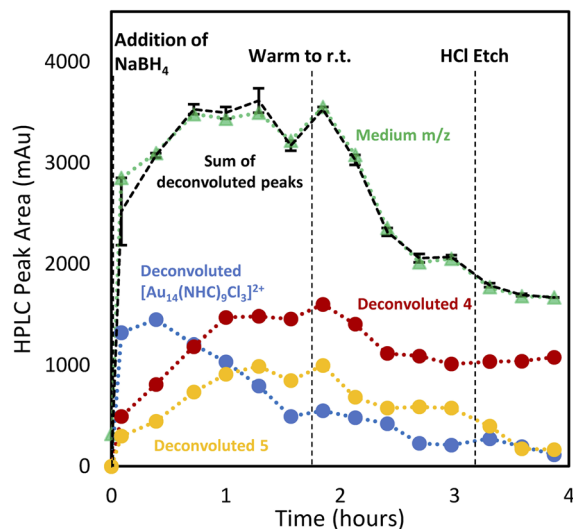
Fig. 5 Peak deconvolution of 8.5–9 min retention time window: red circle (4). Yellow circle (5), blue circle ([Au 14 (NHC) 9 Cl 3 ] 2+ ). Integrated sum for all deconvoluted signals is shown via black dashed line. Error bars indicate the difference between the sum of the deconvoluted peak fit and observed HPLC peak area (green line) for the same 8.5–9 min retention time window.
