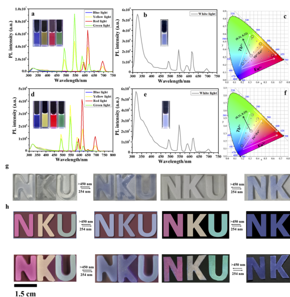
Fig. 6 Emission spectra of different colors (a) blue, green, yellow, red and (b) white doped with different proportions of Tb^{3+} and Eu^{3+} in the H/Ln^{3+}/G_1 assembly in aqueous solution at 298 K (inset: images of luminescence in solution). (c) CIE 1931 chromaticity diagram of the corresponding full-color luminescent coordinates. Emission spectra of different colors (d) blue, green, yellow, red and (e) white doped with different proportions of Tb^{3+} and Eu^{3+} in the H/Ln^{3+}/G_1 assembly in dichloride solution at 298 K (inset: images of luminescence in solution). (f) CIE 1931 chromaticity diagram of the corresponding full-color luminescent coordinates. (g) Under natural light, there is a color change in the letters 'NKU' written (left) by H/Ln^{3+}/G_1 hydrogel and (right) by H/Eu^{3+}/G_1 dichloride solution. (h) Under UV light, there is a change in the luminescent images of the letters 'NKU' written (left) by H/Ln^{3+}/G_1 hydrogel and (right) by H/Eu^{3+}/G_1 dichloride solution (the upper schematic image of changes) ( [H] = 5.0 \times 10^{-5} M).
