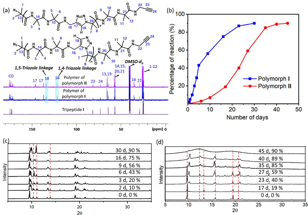
Fig. 4 Characterization of TAAC polymerization. (a) 13 C NMR spectra of polymers of polymorphs I and II (recorded in DMSO-d 6 ) showing the presence of peaks corresponding to both 1,4- and 1,5-triazole linkages. (b) Comparison of kinetic plots for the TAAC reaction of polymorphs I and II. (c and d) Time-dependent PXRD patterns recorded during the polymerization of polymorphs (c) I and (d) II. The peaks which undergo changes are highlighted using a red dashed line.
