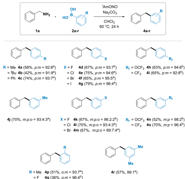
Fig. 3 Arylboronic acid scope of the deaminative coupling between benzylamines and arylboronic acids. Reaction conditions: benzylamine (1a, 2.0 mmol), arylboronic acid (2a-r, 0.5 mmol), isoamyl nitrite (2.5 mmol), sodium carbonate (0.5 mmol), chloroform (1.25 mL), 60 °C, 24 h. Isolated yields after flash column chromatography. a Isomer ratio determined by 13 C NMR. b Isomer ratio determined by 19 F NMR.
