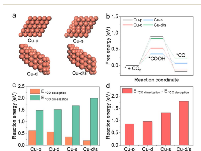
Fig. 4 (a) DFT periodic slab models for Cu(111)-pristine, Cu(111)-dislocation, Cu(111)-step and Cu(111)-dislocation/step structures (denoted as Cu-p, Cu-d, Cu-s and Cu-d/s, respectively). (b) Gibbs free-energy diagrams for the proposed steps of conversion of CO_2 to ^*CO intermediate. (c) Reaction energies for ^*CO desorption to CO and ^*CO coupling to ^*OCCO on Cu catalysts with various defects. (d) Differences in reaction energies for ^*CO coupling to ^*OCCO and ^*CO desorption to CO.
