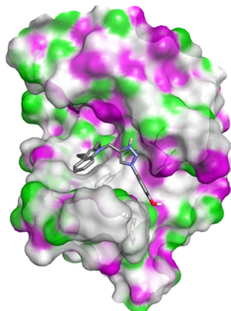
Fig. 6 Docking pose of compound 4q with caspase-3.
