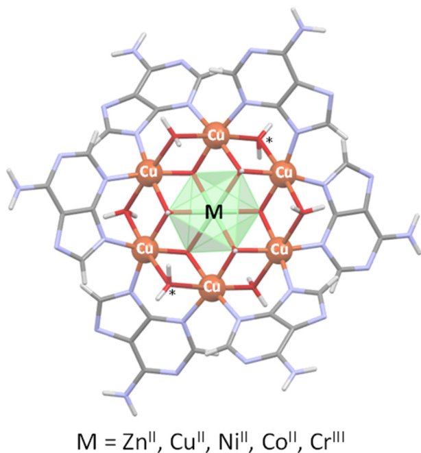
Fig. 1 Heptameric clusters depicting the targeted replacement of the central metal center. Symbol "*" indicates the absent coordination water molecules in compound \text{Cu}_6\text{Cu} .
