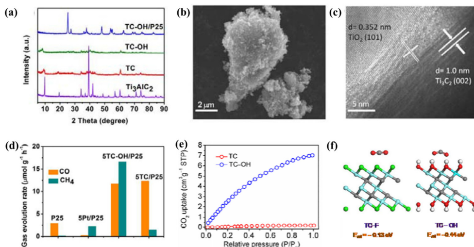
Fig. 7 (a) XRD patterns of Ti 3 AlC 2 , TC, TC-OH particles and TCOH/P25 hybrids. (b) Typical SEM image of the 5TC-OH/P25 mixture. (c) HRTEM images of the interfacial structure of TC-OH and P25 NPs. (d) Under the irradiation of a 300 W xenon lamp, the release rate of CO and CH 4 on P25, 5Pt/P25, 5TC/P25, 5TC-OH/P25. (e) CO 2 adsorption behavior of TC and TC-OH. (f) Side view of CO 2 adsorption models on 2 × 2 × 1 TC-F and 2 × 2 × 1 TC-OH super-cell. Reprinted with permission. 151 Copyright 2018, John Wiley and Sons.
