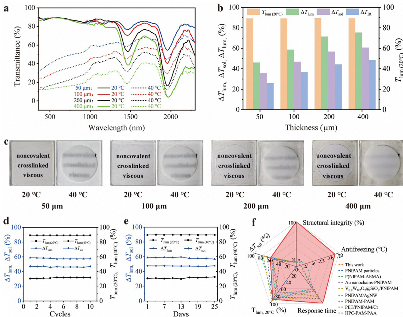
Fig. 4 (a) Transmittance spectra for 50, 100, 200, and 400 μm at 20 °C (solid line) and 40 °C (dashed line), respectively. (b) Comparison of optical performance ( T_{lum}(20^{\circ}\text{C}) , \Delta T_{lum} , \Delta T_{sol} and \Delta T_{IR} ) for the 50, 100, 200, and 400 μm smart windows. (c) Optical photos for the 50, 100, 200, and 400 μm sample at 20 °C and 40 °C, respectively. Cycling testing (d) and long-term stability testing (e) for the 100 μm sample. (f) Comparison of this work with the recently reported results of covalent crosslinked hydrogel-based thermochromic windows regarding the performance evaluation parameters.
