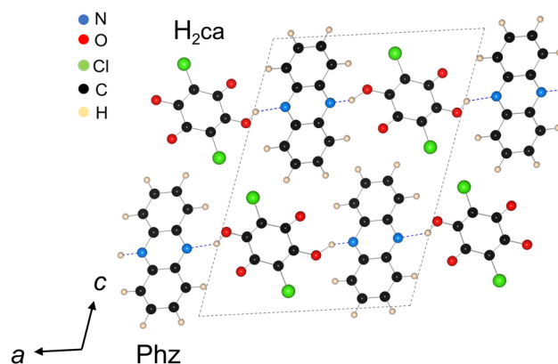
Fig. 1 Molecular structures for Phz and H 2 ca and crystal arrangement viewed along the b -axis in the ferroelectric phase. 20
