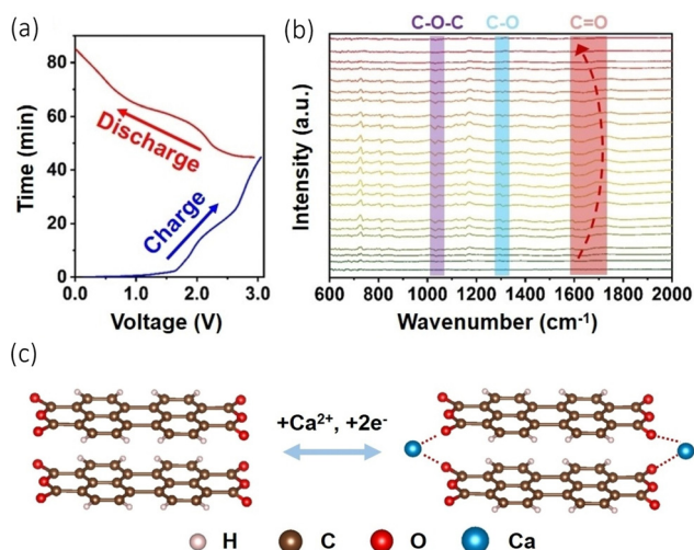
Fig. 6 (a) Charge/discharge curves of PTCDA/graphite cathode during in situ test. (b) In situ FT-IR spectra for the PTCDA anode. (c) Suggested electrochemical conversion of PTCDA with \text{Ca}^{2+} insertion/de-insertion. Reproduced with permission from ref. 82, copyright Wiley-VCH.
