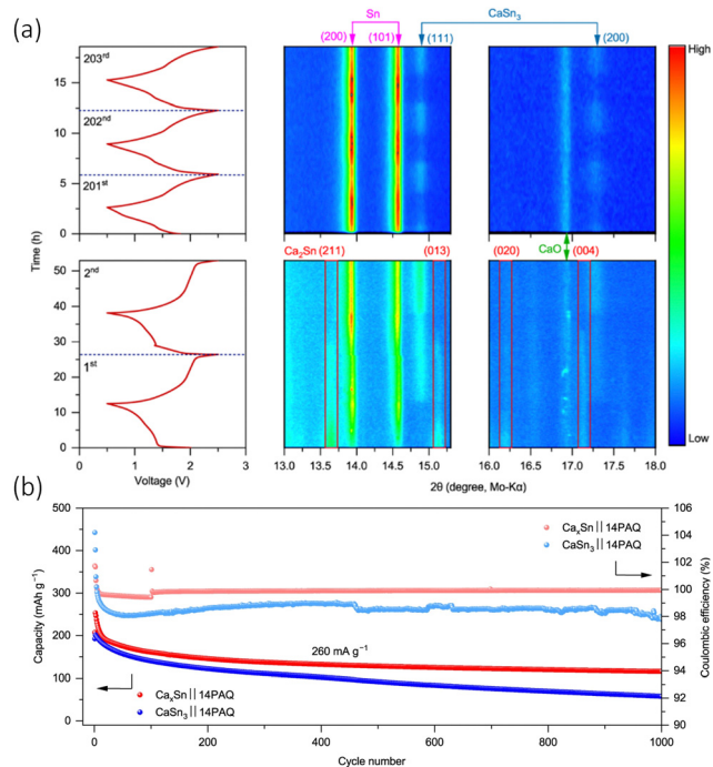
Fig. 8 (a) Isoplots of in situ XRD scans the anode \text{Ca}_x\text{Sn}||14\text{PAQ} cells during the first, second and from 201st to 203rd discharge/charge cycles at specific current of 26 \text{ mA g}^{-1} at 25^\circ\text{C} . The peak is observed along the top and the cell voltage profiles on the left had side. ICSD-ID: \text{Ca}_2\text{Sn} 659 611, \beta\text{-Sn} 106 072, \text{CaSn}_3 58 934, \text{Ca}_{36}\text{Sn}_{23} 54 619 and \text{CaO} 26 959. (b) Cycling performance of \text{CaSn}_3||14\text{PAQ} compared with \text{Ca}_x\text{Sn}||14\text{PAQ} . Reproduced with permission from ref. 94, copyright 2022 Springer Nature.
