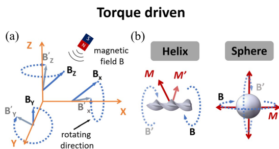
Fig. 6 (a) Schematic of rotating magnetic field actuation. The magnetic fields can rotate around three axes of the coordinate to achieve 3D actuation. (b) There are two typical motion modes, helix and sphere, which show different motion modes under the rotating magnetic fields.
