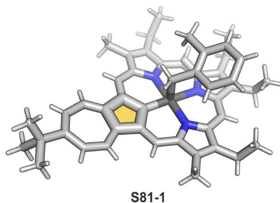
Fig. 19 Axial and equatorial organometallic rhodium(III) complexes of azuliporphyrin.
