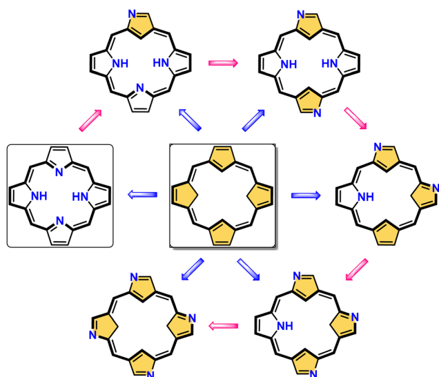
Scheme 133 Complementary strategies: inner core/perimeter four nitrogen atom nitriding of quaterpyrrole (blue arrows) and stepwise N-confusion of regular porphyrin (blue arrow nitriding and purple arrow N-confusion).
