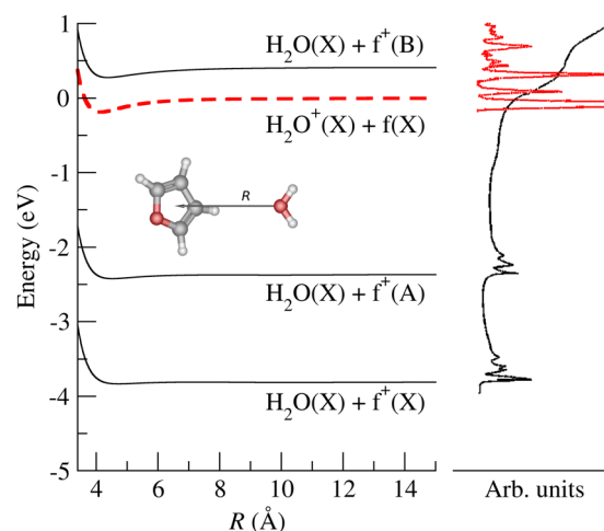
Fig. 5 Potential energy curves for the four lowest electronic states of the (\text{furan} + \text{H}_2\text{O})^{+\bullet} system, as a function of the interfragment distance, R . The asymptotic fragments are indicated for each channel. Photoelectron spectra for furan (black line) and \text{H}_2\text{O} (red line) are included for comparison with the ab initio PEC. f^+ stands for \text{furan}^{+\bullet} .
