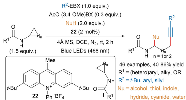
Scheme 39 Photoredox-catalyzed alkynylative ring-opening of cycloalkylamides.
