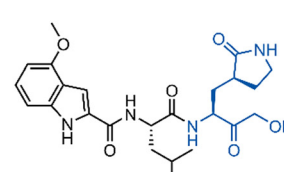
49 (PF-00835231) SARS-CoV-2 EC_{50} = 231 nM
