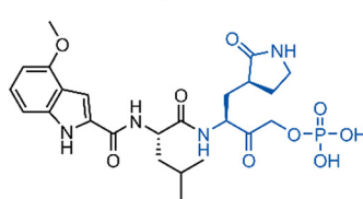
50 (Lufotrelvir, PF-07304814) SARS-CoV-2 K_i = 174 nM, EC_{50} = 86.7 nM
