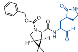
48 SARS-CoV-2 IC_{50} = 54 nM, EC_{50} = 0.37 \mu M
