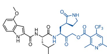
44 SARS-CoV-2 IC_{50} = 0.017 \mu M, EC_{50} = 0.28 \mu M
