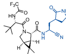
51 (Nirmatrelvir, PF-07321332) SARS-CoV-2 EC_{50} = 74.5 nM
