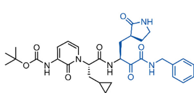
43 SARS-CoV-2 IC_{50} = 670 nM, EC_{50} = 1.8 \mu M
