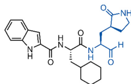
46 SARS-CoV-2 IC_{50} = 53 nM
