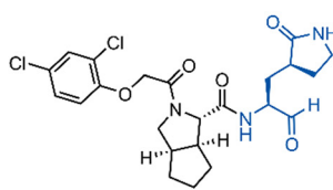
47 (MI-30) SARS-CoV-2 IC_{50} = 17 nM, EC_{50} = 0.54 \mu M
