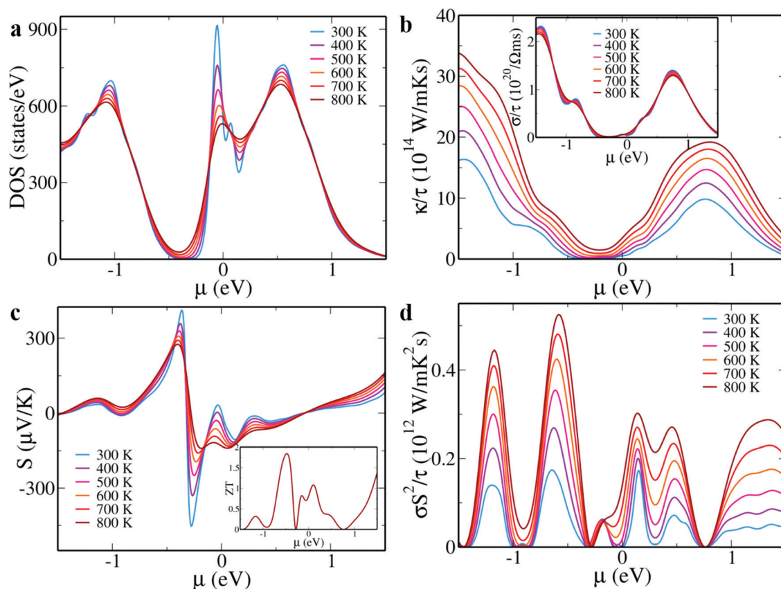
Fig. 2 (a) DOS; (b) thermal conductivity (inset: electrical conductivity); (c) Seebeck co-efficient (inset: ZT at 800 K) and (d) power factor of \text{Sn}_{15}\text{MoTe}_{16} as functions of chemical potential ( \mu ) at various temperatures. Conductivity and power factor values are reported by scaling them with \tau .
