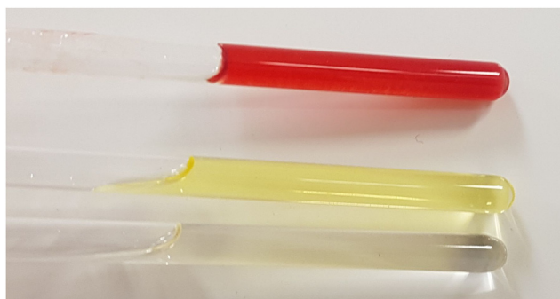
Fig. 2 Top. Donor-acceptor organogel obtained from C 3 Pyr and C 3 NDI in TCE- d 2 ([ C 3 Pyr ] = [ C 3 NDI ] = 5.2 mM). Middle. Solution of C 3 NDI in TCE (5.2 mM). Bottom. Solution of C 3 Pyr in TCE (5.2 mM).
