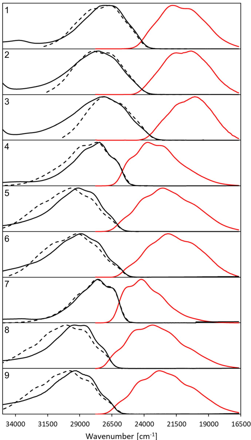
Fig. 2 Normalized, corrected absorption (solid black line), fluorescence (solid red line) and mirror-image of fluorescence spectra (dashed black line) shifted to match the 0–0 point in CHCl 3 .
