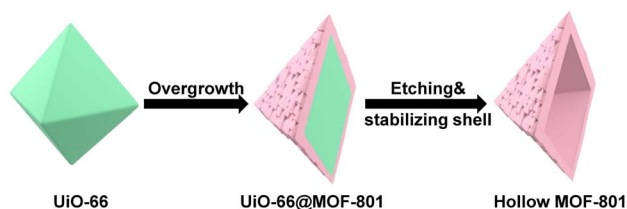
Scheme 1 Scheme of the synthesis of hollow MOF-801.
