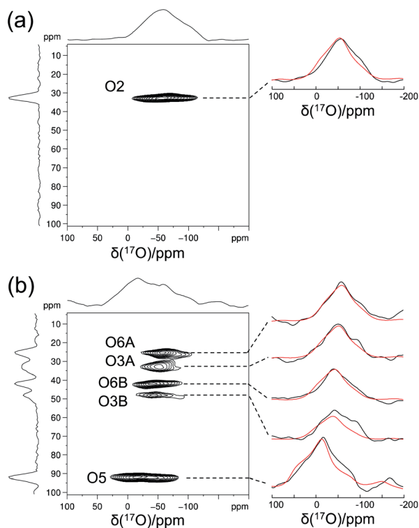
Fig. 7 2D ^{17}\text{O} 3QMAS spectra of (a) [2\text{-}^{17}\text{O}]\text{-}\alpha\text{-D-glucose} and (b) [3/5/6\text{-}^{17}\text{O}]\text{-}\alpha\text{-D-glucose} obtained at 18.8 T with a Bruker 3.2 mm CPMAS CryoProbe. The sample spinning frequency was 15 kHz. Each sample contains 10% (w/w) Cu-EDTA. Experimental (black traces) and simulated (red traces) F2-slice spectra are displayed on the side. Data acquisition parameters are: (a), recycle delay 1 s, 48 t_1 increments (with apodization weighted sampling, n_0 = 1536 transients), total experimental time 10 h; (b) recycle delay 1 s, 32 t_1 increments (with apodization weighted sampling, n_0 = 31\,680 transients), total experimental time 6 days.
