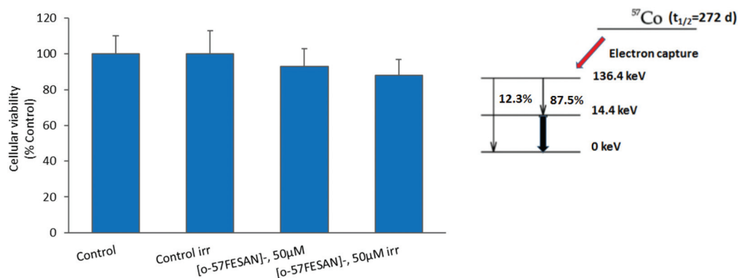
Fig. 8 Cellular viability of U87 GBM cells after irradiation with X-rays in the presence of 50 μM Na[o- 57 FESAN]. Irradiation was done using a Philips MCN 165 X-ray tube and a YXLON 9421 high-voltage generator at a 0.4 mGy radiation dose. ISO beam quality N120 was used ( E_{\text{max}} = 120 keV, E_{\text{ave}} = 100 keV, filtered with 4 mm Al + 5 mm Cu + 1 mm Sn).
