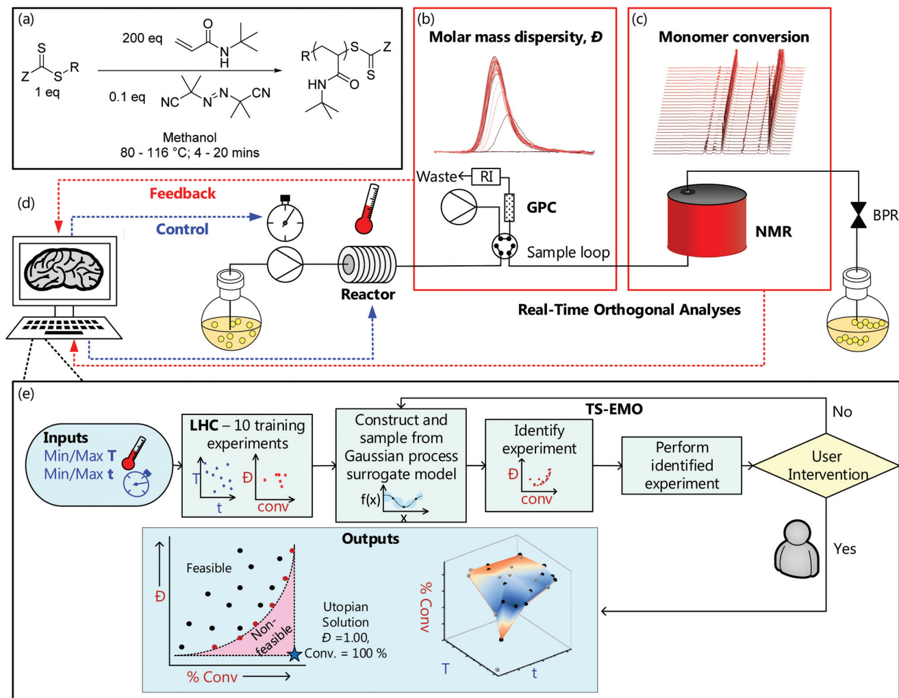
Fig. 1 (a) Generalised scheme for the RAFT synthesis of \text{P}(\text{tBuAm})_{200} . Example (b) gel permeation chromatography (GPC) chromatograms and (c) ^1\text{H} nuclear magnetic resonance (NMR) spectra from the automated continuous flow platform used in this work (see ESI† for full platform details and all analytical data). (d) Schematic of that automated platform and (e) an overview of the structure of the machine learning directed (Thompson-sampling efficient multi-objective optimisation (TSEMO) algorithm) experiments used in this work.
