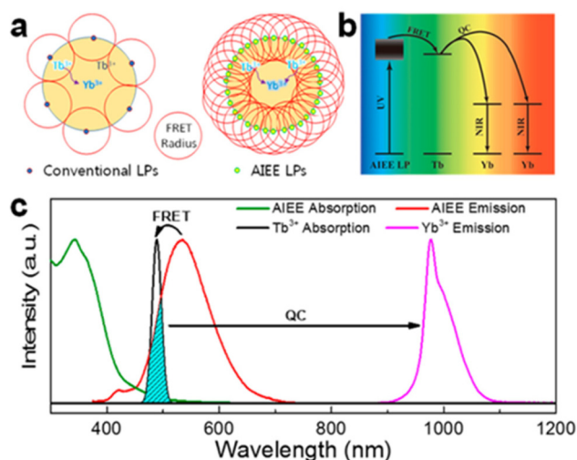
Fig. 7 (a) Schematic illustration of the difference between conventional emission and AIE in the sensitization of quantum cutting. (b) Energy-transfer pathway from the AIEE LPs to NPs. (c) Normalized absorption and photoluminescence spectra of the AIEE dye and NPs. Reprinted with permission from ref. 125. Copyright (2018) American Chemical Society.
