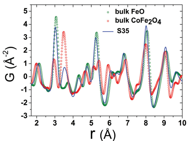
Fig. 6 Representative low- r raw data collected at T = 300 K for reference materials \text{FeO} (green circles), \text{CoFe}_2\text{O}_4 (red circles) and the \text{FeO}@CoFe_2\text{O}_4 nanocrystal sample S35 (blue line). The normalization is realized by dividing the x -PDF patterns with the intensity of the peak centered at \sim 2.0 Å (first peak, attributed to nearest-neighbour Fe–O pairs). The various contributions of the two different crystallographic phases, represented here by the bulk reference samples, account for slight peak shifts and, in some cases, variations of peak intensities of the experimental PDFs in the NCs. For clarity, only data for nanocrystal sample S35 are shown here, whereas data for the remaining NCs (S12, S21) are compared in Fig. 7.
