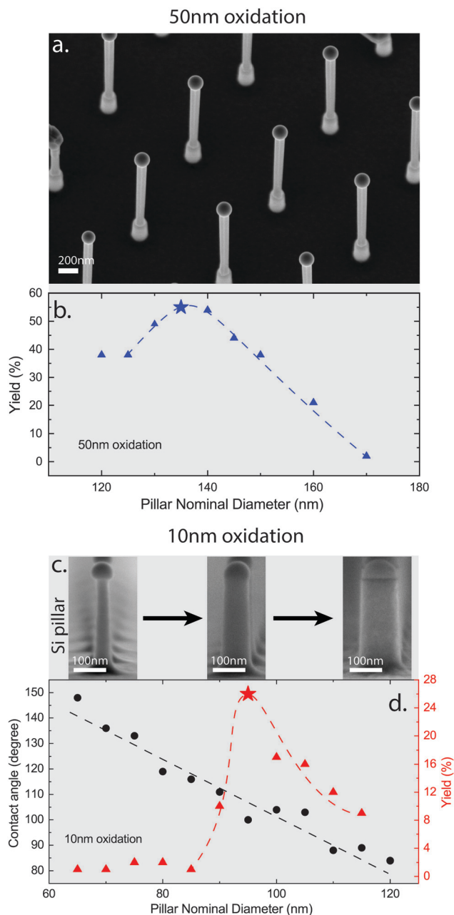
Fig. 2 Aspects and statistics of NW growths done on EBL-patterned \text{SiO}_2/\text{Si} pillars. (a) SEM image ( 20^\circ tilt) showing vertical GaAs NWs grown on \text{SiO}_2/\text{Si} (111) pillars. (b) Vertical yield as a function of pillar nominal diameter. (c) SEM images showing Ga droplets on top of \text{SiO}_2/\text{Si} pillars of different nominal diameters. (d) Contact angle and yield as a function of pillar nominal diameter for pillars as shown in c. The optimum contact angle is identified as the one showing the best vertical yield.
